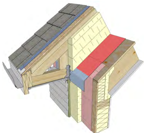
Sheathing Membrane
