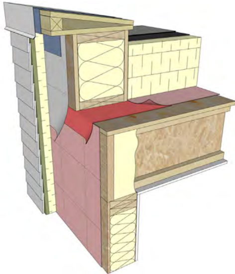
Parapet Pre-Strip
