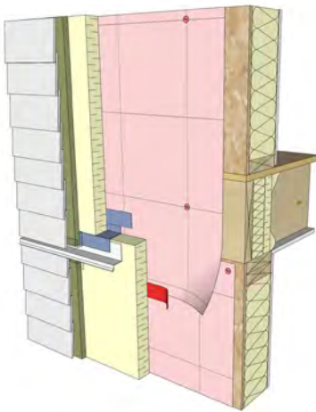
Sheathing Membrane
