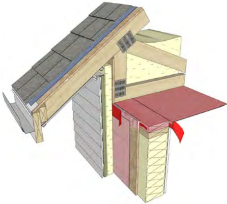
Sheathing Sealant
