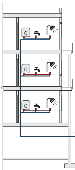
In-suite tankless hot water heaters
