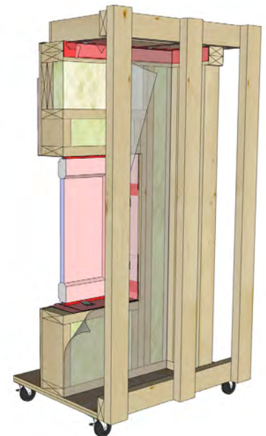
2x4 framing for horizontal transport
