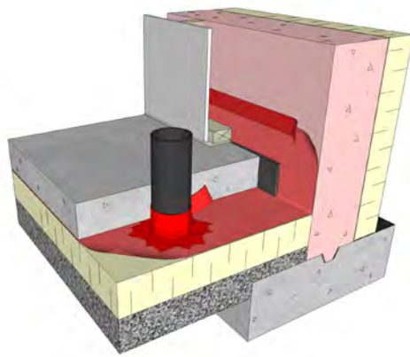
Taped Membrane
