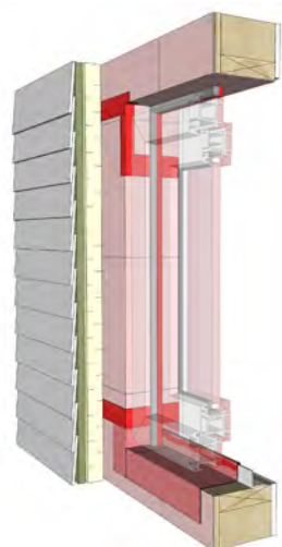
Back-dam
